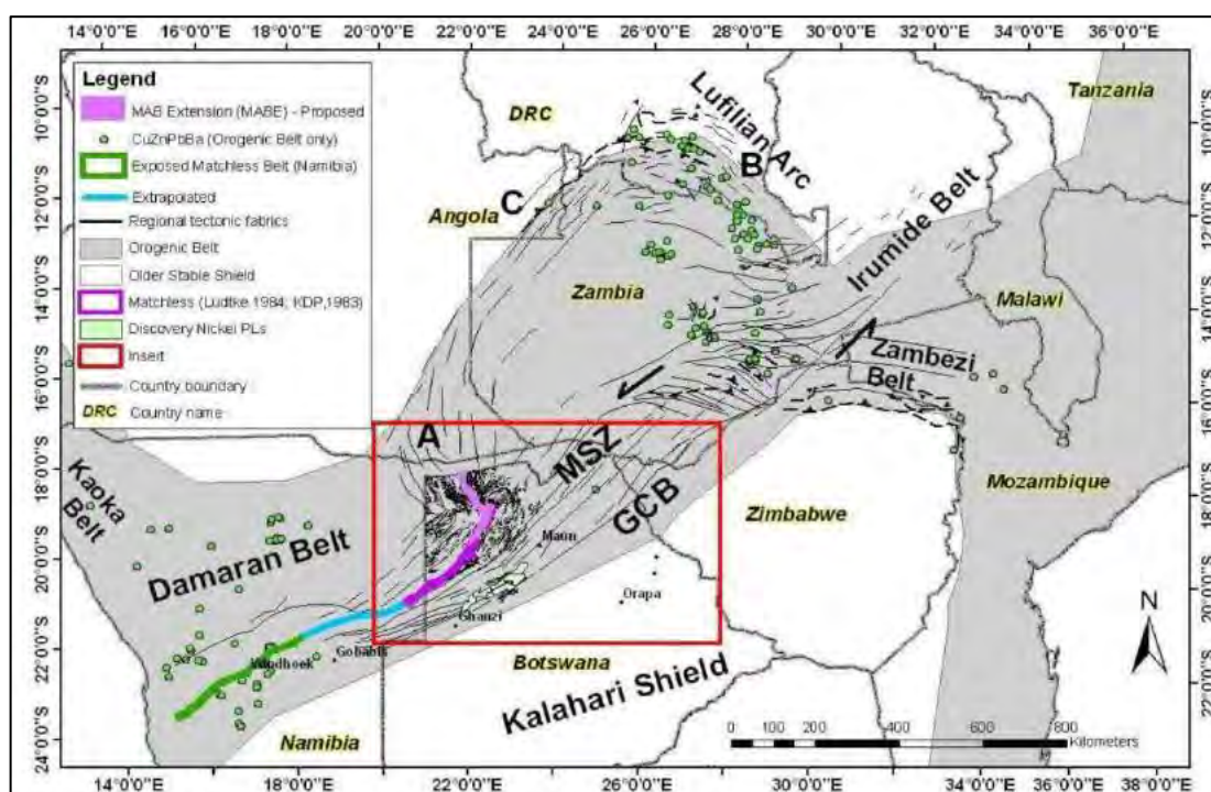
Figure 6-2: Southern African Orogeny tectonic map*. Red insert - Figure 6-3 (Source: De Wit, 2009).
