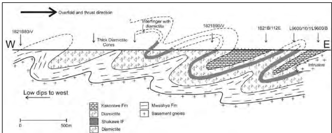
Figure 6-7: Geological cross-section in Shakawe area* (Source: Beukes, 2012)
